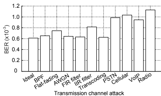
Fig. 12 Overall system robustness tests in the presence of various transmission channel attacks at a bit rate of 200 bits/s
