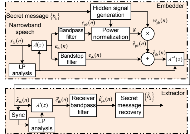
Fig. 3 Overall system design for narrowband speech watermarking
